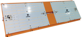
1. Board 240W WIDE UV+IR
